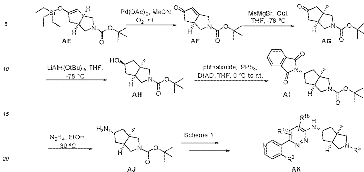
Scheme 9
