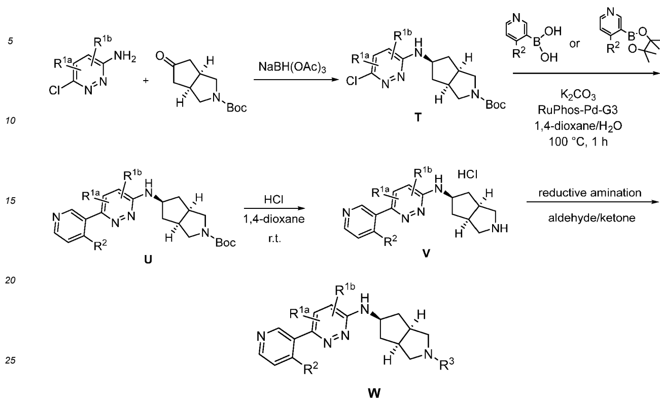
Scheme 7
