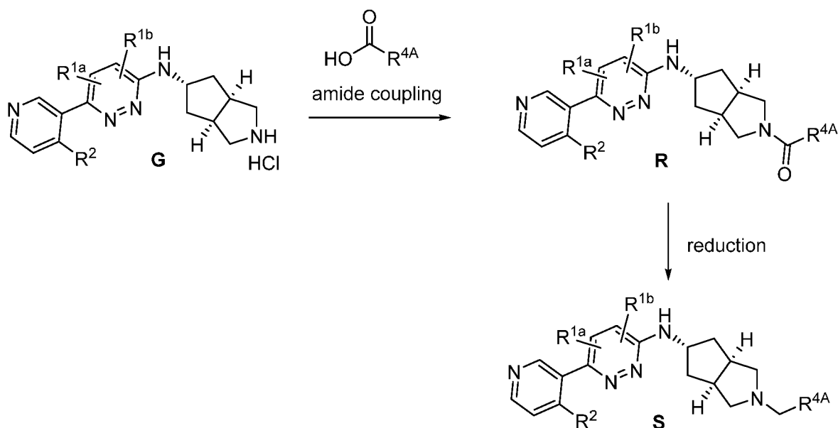
Scheme 6
