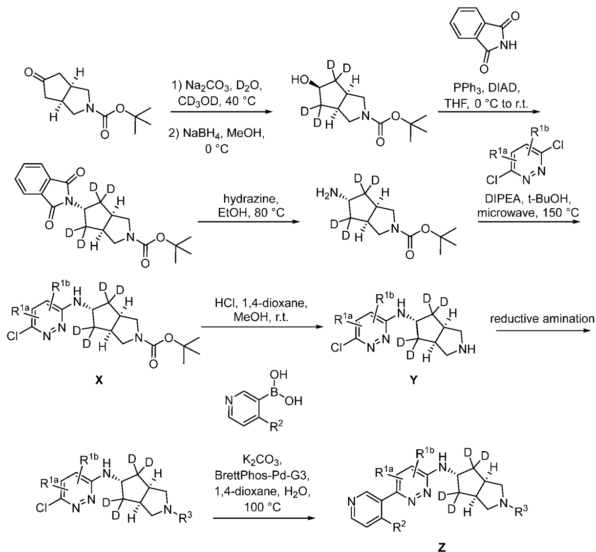
Scheme 8
