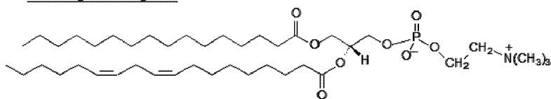
1-hexadecanoyl-2-linoleoyl-sn-glycero-3-phosphocholine
