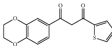
1-(2,3-dihydrobenzo[b][1,4]dioxin-6-yl)-3-(thiophen-2-yl)propane-1,3-dione 16
