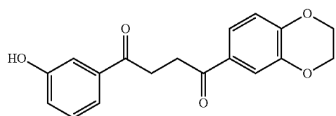
1-(2,3-dihydrobenzo[b][1,4]dioxin-6-yl)-4-(3-hydroxyphenyl)butane-1,4-dione 6
