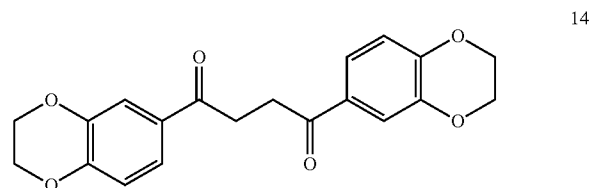
1,4-bis(2,3-dihydrobenzo[b][1,4]dioxin-6-yl)butane-1,4-dione 14
