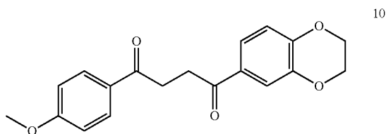
1-(2,3-dihydrobenzo[b][1,4]dioxin-6-yl)-4-(4-methoxyphenyl)butane-1,4-dione 10
