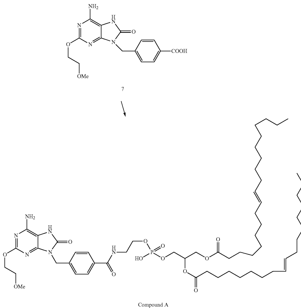
Preparation of compound A
