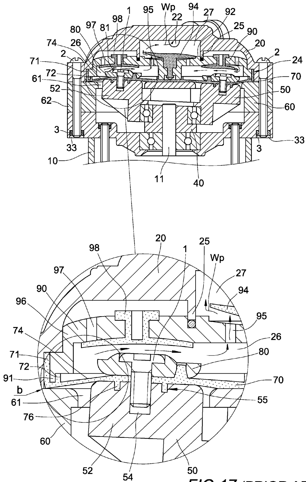
FIG. 17 (PRIOR ART)
