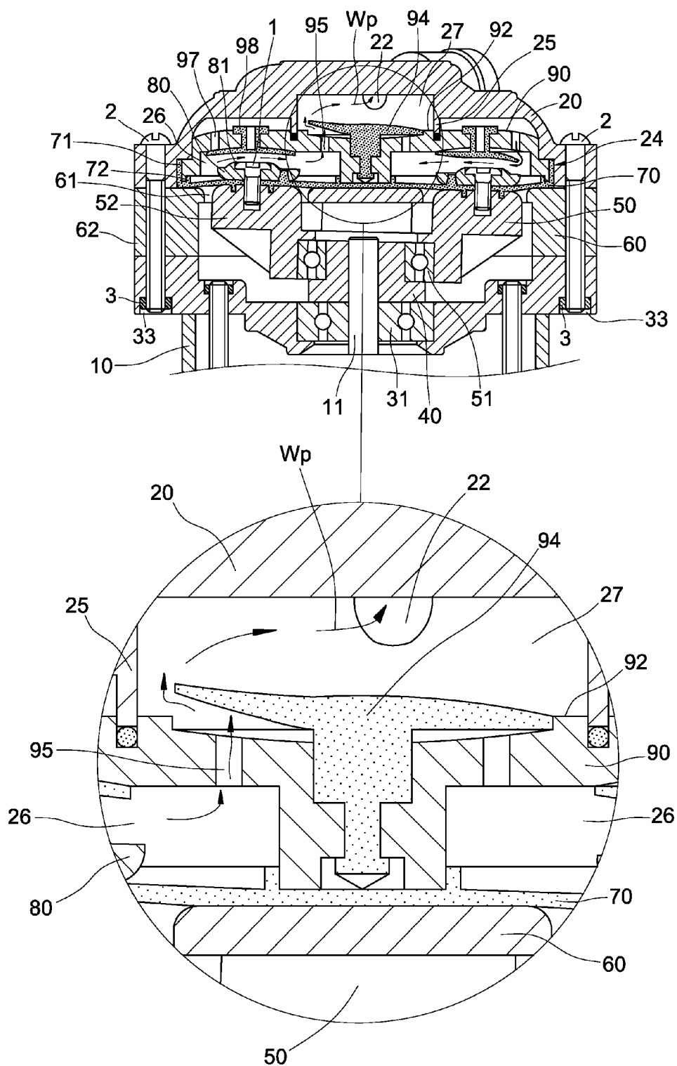
FIG.13 (PRIOR ART)
