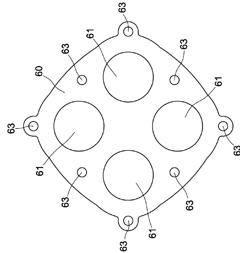
FIG. 7 (PRIOR ART)
