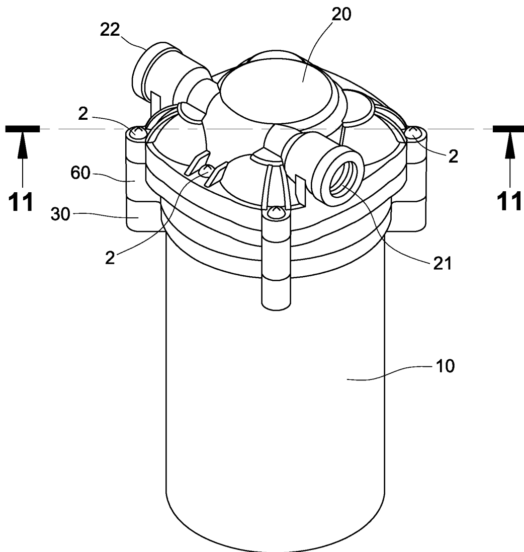
FIG. 1 (PRIOR ART)
