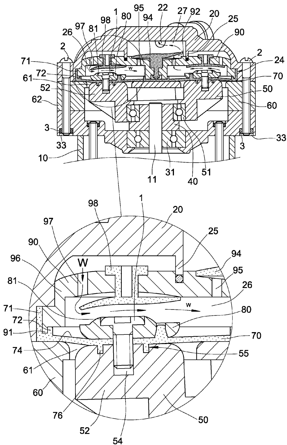
FIG. 12 (PRIOR ART)
