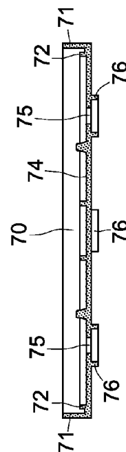
FIG. 9 (PRIOR ART)
