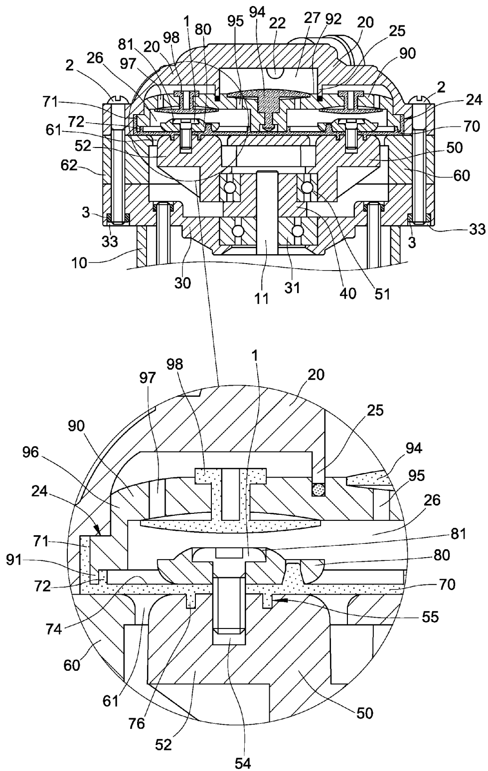
FIG.11 (PRIOR ART)
