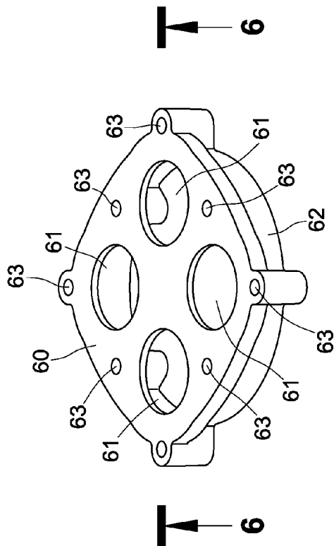
FIG. 5 (PRIOR ART)
