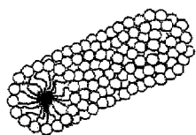
ROD-LIKE MICELLE
