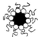
REVERSE MICELLE
