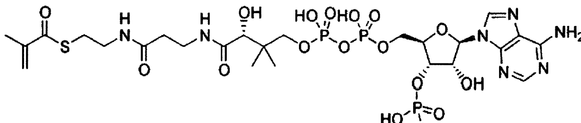
[Chem 1]
