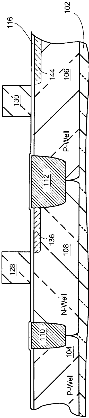
FIG. 2D (PRIOR ART)
