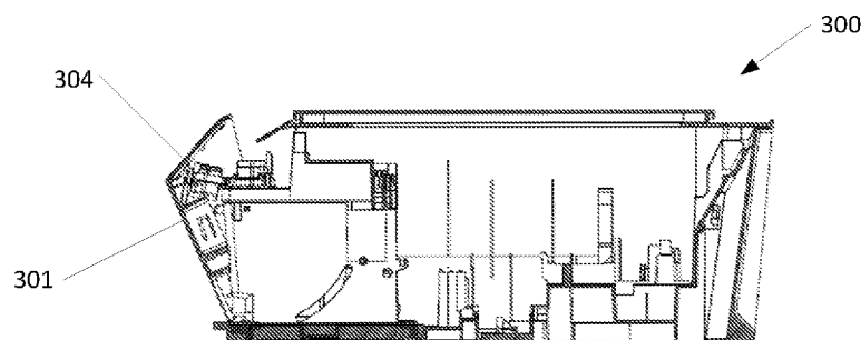
Figure 17 (section A-A)
