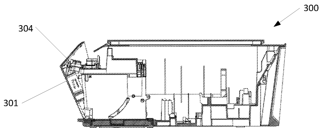
Figure 17 (section A-A)
