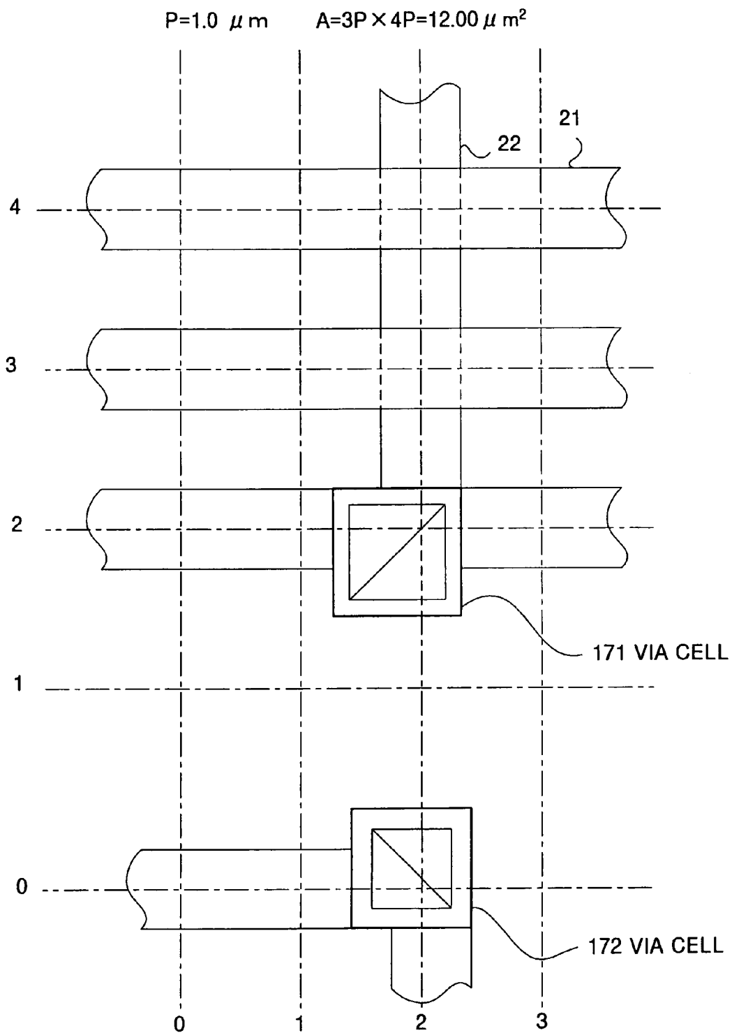
(PRIOR ART) FIG. 17
