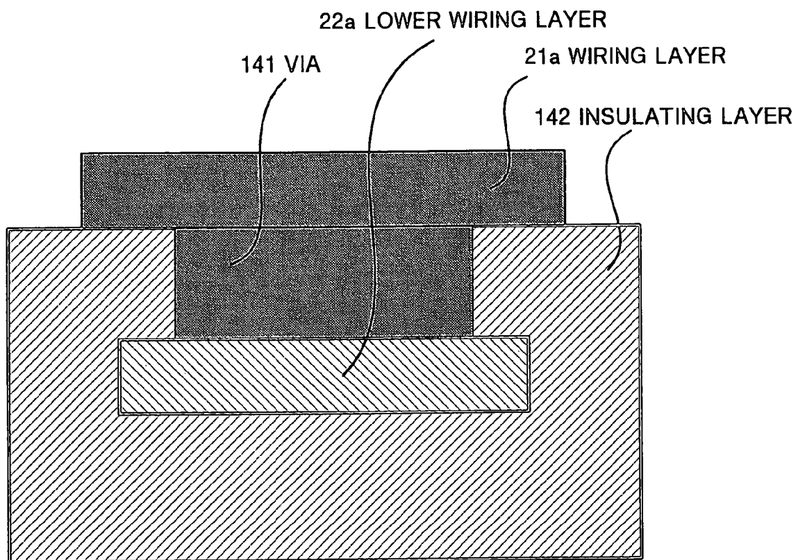
FIG. 14B (PRIOR ART)
