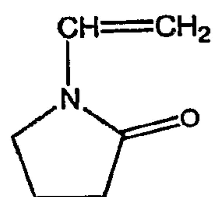
Vinyl pyrrolidone
