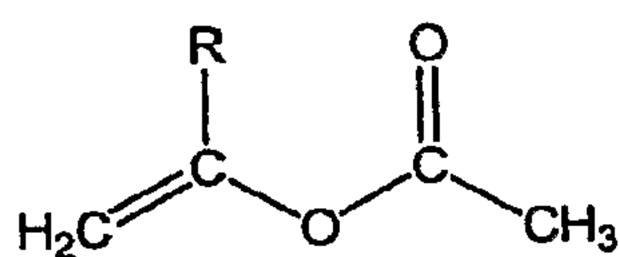
Vinyl Acetate
