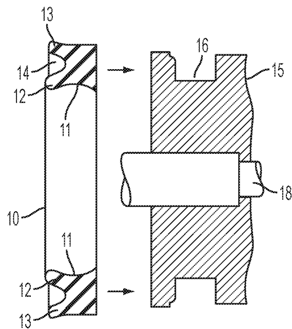
FIG. 2 PRIOR ART
