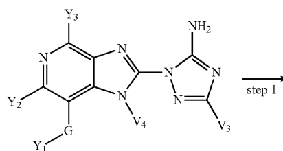
Scheme 8
