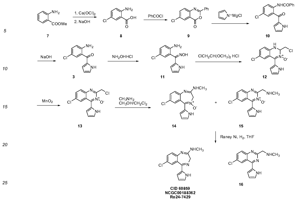
Scheme 1. Synthesis of Ro24-7429
