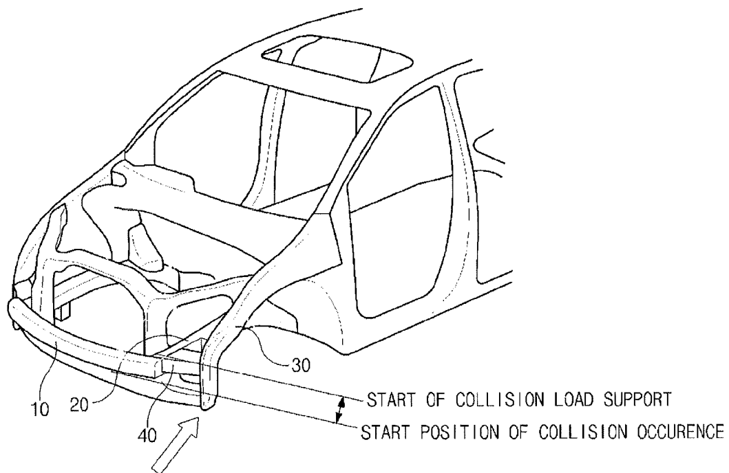
FIG. 1 (Related Art)
