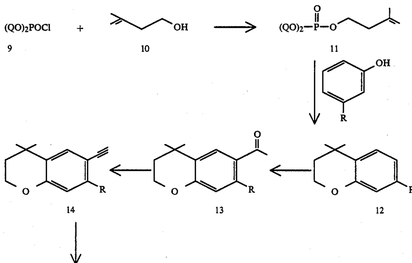
Reaction Scheme II
