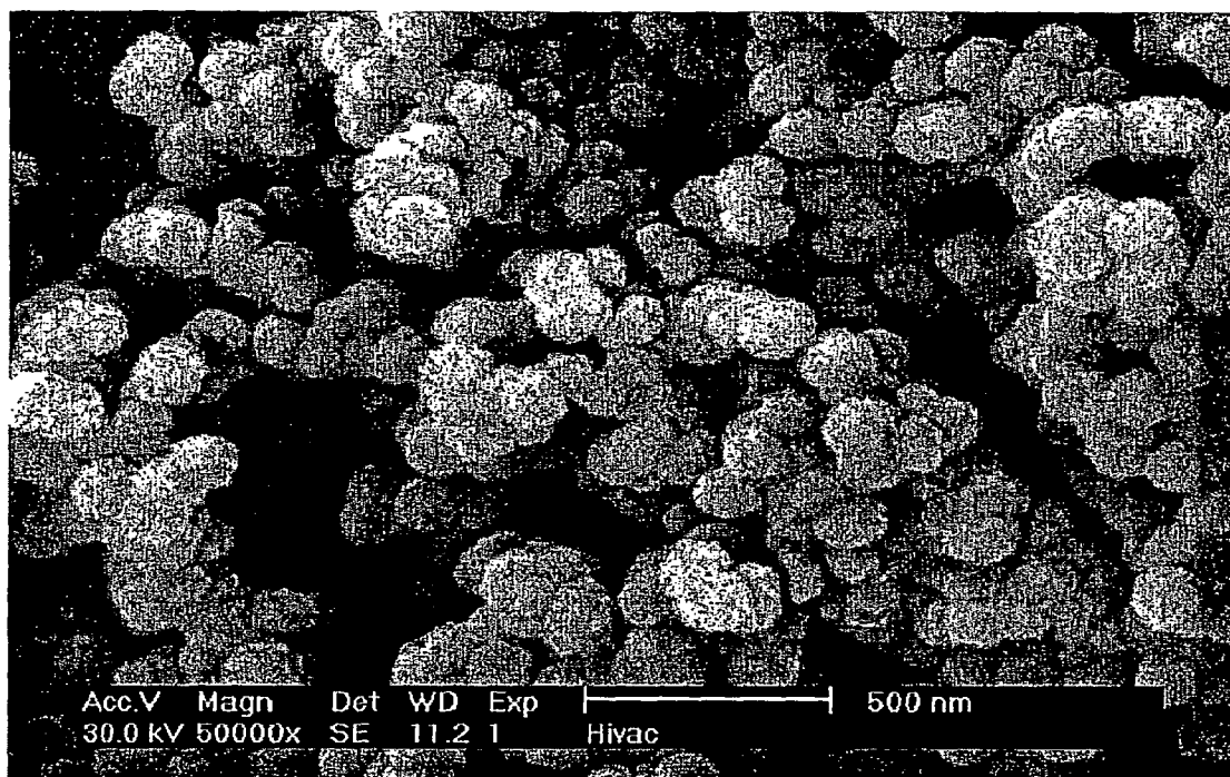
Figure 5: SEM image, at 50,000x, of product of LPD silica reaction with fullerenol added to reaction mixture.
