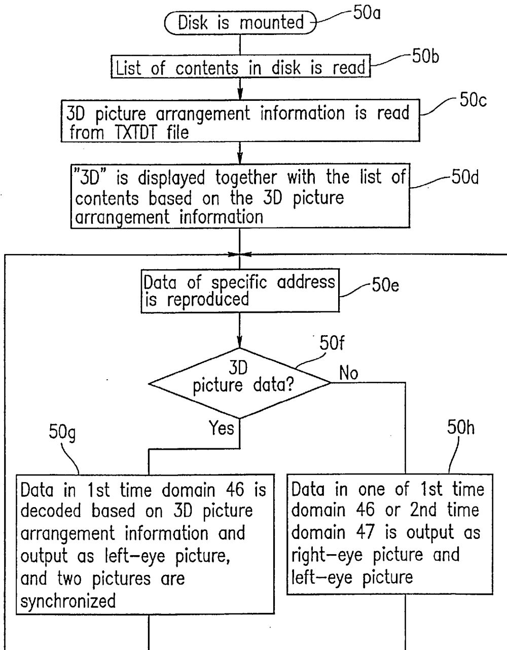
Operation flowchart of 3D picture reproduction apparatus
