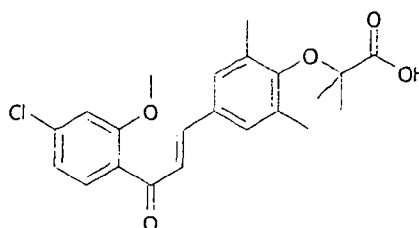
1-[2-methoxy-4-chlorophenyl]-3-[3,5-dimethyl-4-carboxydimethylmethoxyphenyl]prop-2-en-1-one
