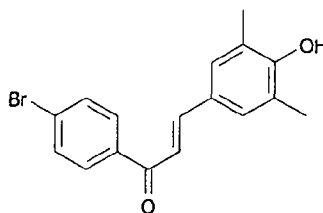
1-[4-bromophenyl]-3-[3,5-dimethyl-4-hydroxyphenyl]prop-2-en-1-one (Compound 16)
