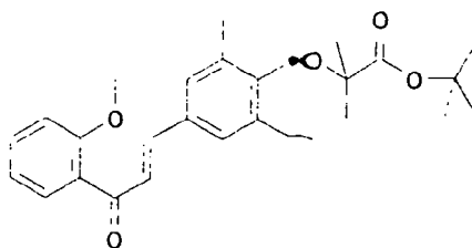
1-[2-methoxyphenyl]-3-[3,5-dimethyl-4-tert-butylloxycarbonyldimethylmethoxyphenyl]prop-2-en-1-one (Compound 5)
