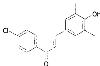
1-[4-chlorophenyl]-3-[3,5-dimethyl-4-hydroxyphenyl]prop-2-en-1-one (Compound 1)
