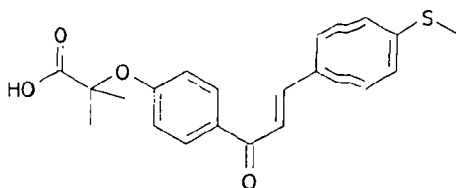
1-[4-carboxydimethylmethoxyphenyl]-3-[4-methylthiophenyl]prop-2-en-1-one
