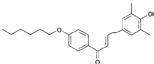
1-[4-hexyloxyphenyl]
