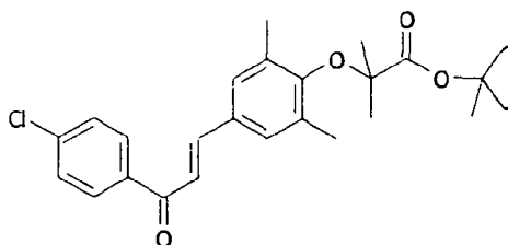
1-[4-chlorophenyl]-3-[3,5-dimethyl-4-tert-butyloxycarbonyldimethylmethoxyphenyl]prop-2-en-1-one (Compound 2)
