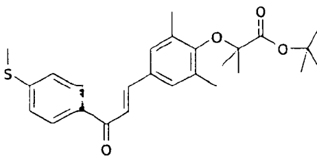
1-[4-methylthiophenyl]-3-[3,5-dimethyl-4-tert-butylloxycarbonyldimethylmethoxyphenyl]prop-2-en-1-one (Compound 8)
