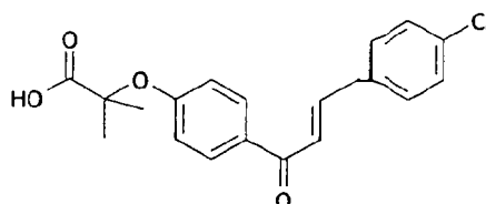
1-[4-carboxydimethylmethylthiophenyl]-3-[4-methylthiophenyl]prop-2-en-1-one
