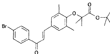
1-[4-bromophenyl]-3-[3,5-dimethyl-4-tert-butylmethoxyphenyl]prop-2-en-1-one (Compound 17)
