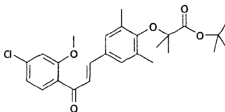
1-[2-methoxy-4-chlorophenyl]-3-[3,5-dimethyl-4-carboxydimethylmethoxyphenyl]prop-2-en-1-one
