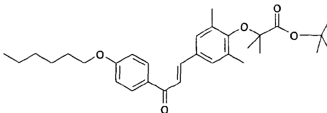
5 1-[4-hexyloxyphenyl]-3-[3,5-dimethyl-4-carboxydimethylmethoxyphenyl]prop-2-en-1-one
