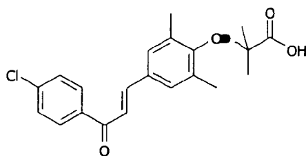
5 1-[4-methylthiophenyl]-3-[4-carboxydimethylmethoxyphenyl]prop-2-en-1-one
