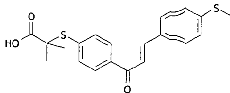
1-[4-carboxydimethylmethoxyphenyl]-3-[4-methylthiophenyl]prop-2-en-1-one
