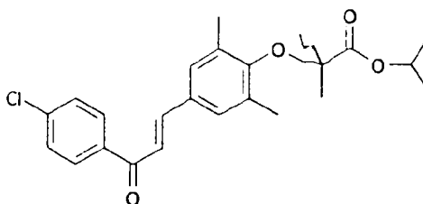
1-[4-chlorophenyl]-3-[3,5-dimethyl-4-carboxydimethylmethoxyphenyl]prop-2-en-1-one
