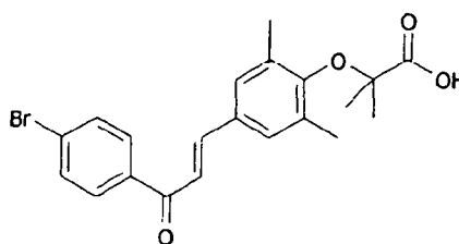
1-[4-bromophenyl]-3-[3,5-dimethyl-4-carboxydimethylmethoxyphenyl]prop-2-en-1-one (Compound 18)
