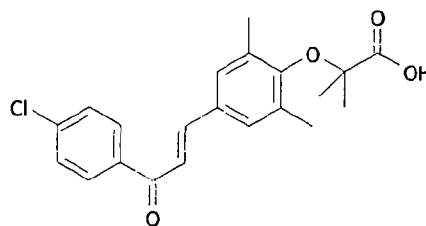
1-[4-chlorophenyl]-3-[3,5-dimethyl-4-carboxydimethylmethoxyphenyl]prop-2-en-1-one (Compound 3)
