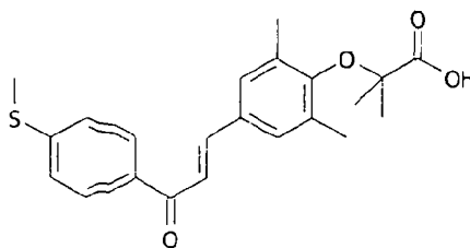
1-[4-methylthiophenyl]-3-[3,5-dimethyl-4-carboxydimethylmethoxyphenyl]prop-2-en-1-one (Compound 9)
