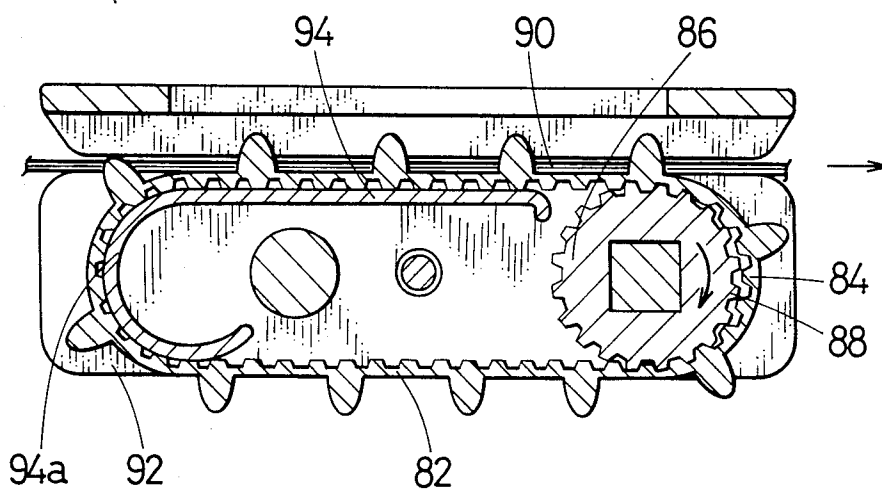
FIG. 17 (PRIOR ART)
