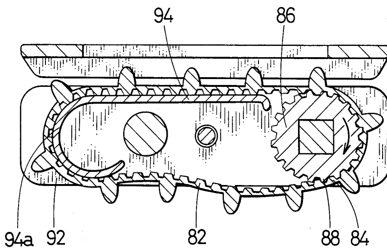
FIG. 16 (PRIOR ART)
