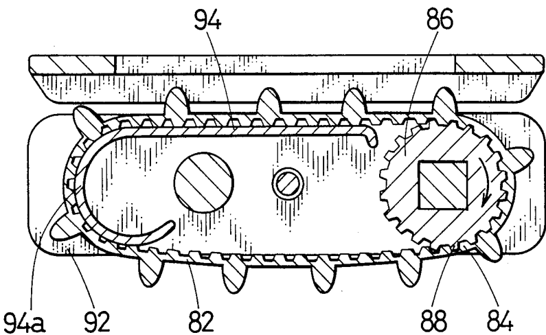
FIG. 14 (PRIOR ART)
