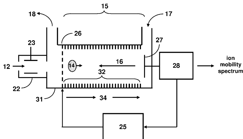
ion mobility spectrometer with virtual aperture grid (30)
