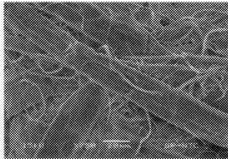
FIG. 2B 25% MICROFIBER, YANKEE SIDE
