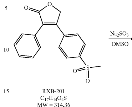
Scheme 2. Formation of 4-[4-(methylsulphonyl)phenyl]-3-phenyl-5-hydroxyfuran-2-one(RXB-Hydroxy) impurity
