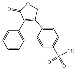
Chemical Structure of Rofecoxib
