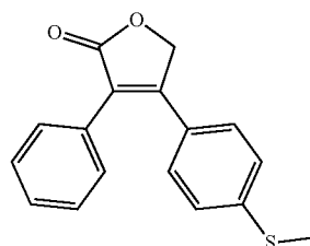
Stage 3 RXB-Furanone C_{17}H_{14}O_2S MW = 282.36
