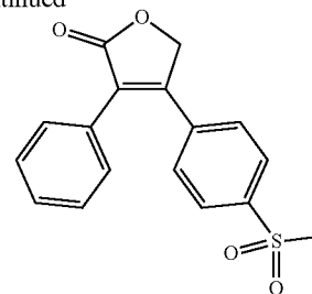
Stage 4 crude RXB-201 C_{17}H_{14}O_4S MW = 314.36
