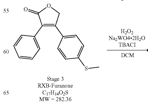
Scheme 4. Oxidation of 4-[4-(methylthio)phenyl]-3-phenyl-2(5H)-furanone in DCM/H 2 O
