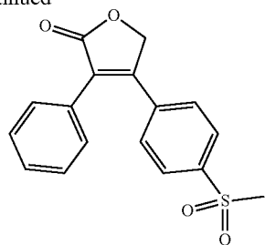
Stage 4 crude RXB-201 C_{17}H_{14}O_4S MW = 314.36
