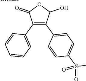
RXB-Hydroxy C 17 H 14 O 5 S MW = 330.36
