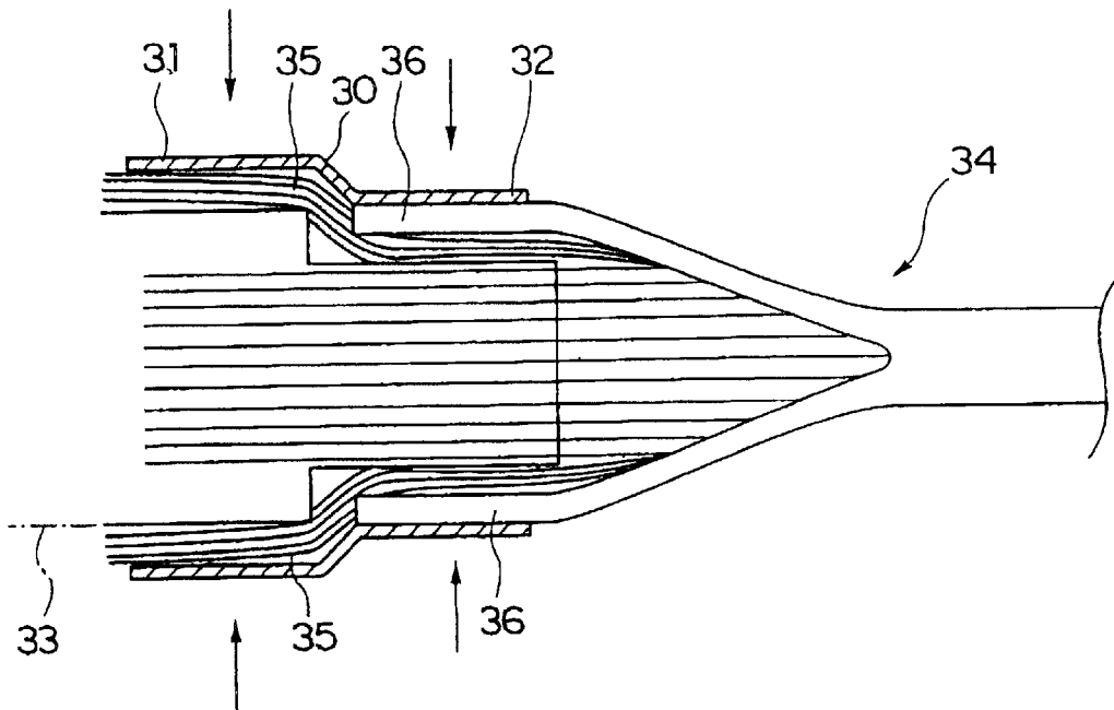
FIG. 6 PRIOR ART
