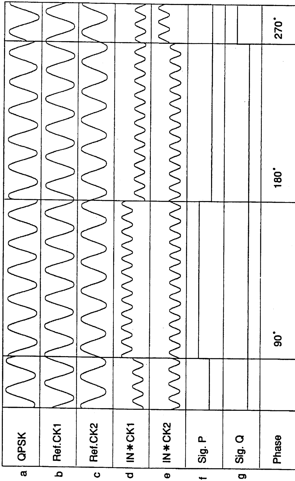
TIMING CHART OF CONVENTIONAL DEMODULATION CIRCUIT
