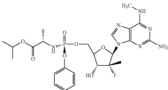
Compound 5-2 (Table 7)
