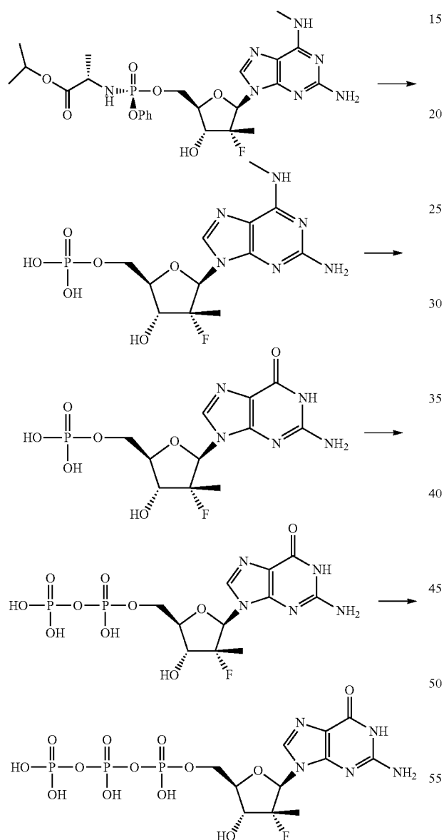
Scheme 1
