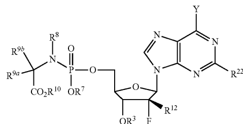
Formula III
