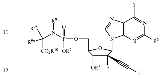
Formula V
