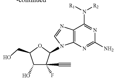
Target compound
