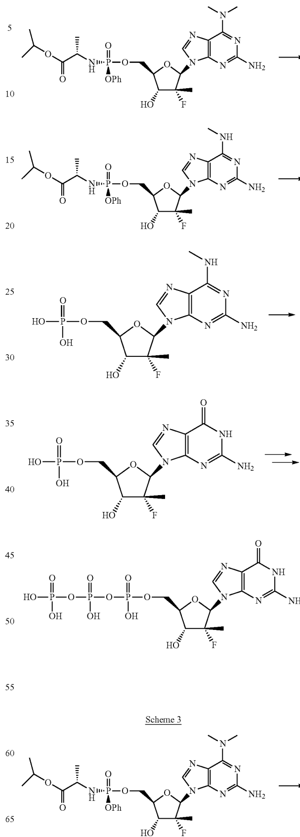
Scheme 2
