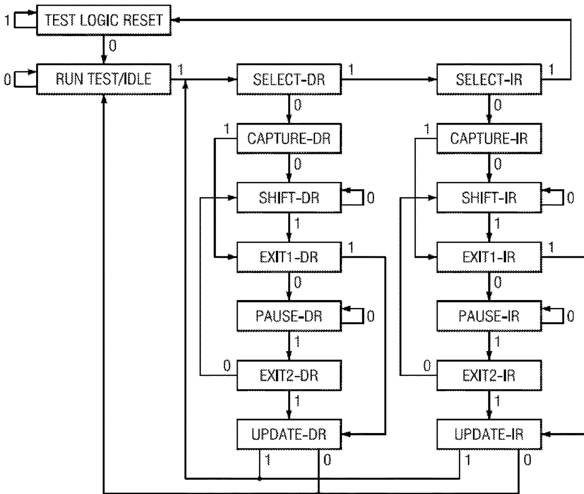
FIG. 2 (PRIOR ART)
