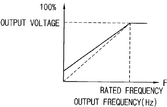
FIG. 3B CONVENTIONAL ART
