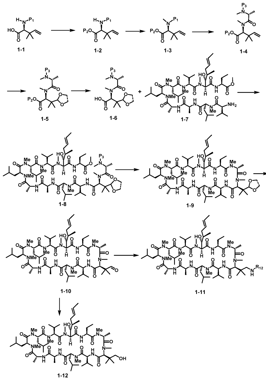
Scheme 1
