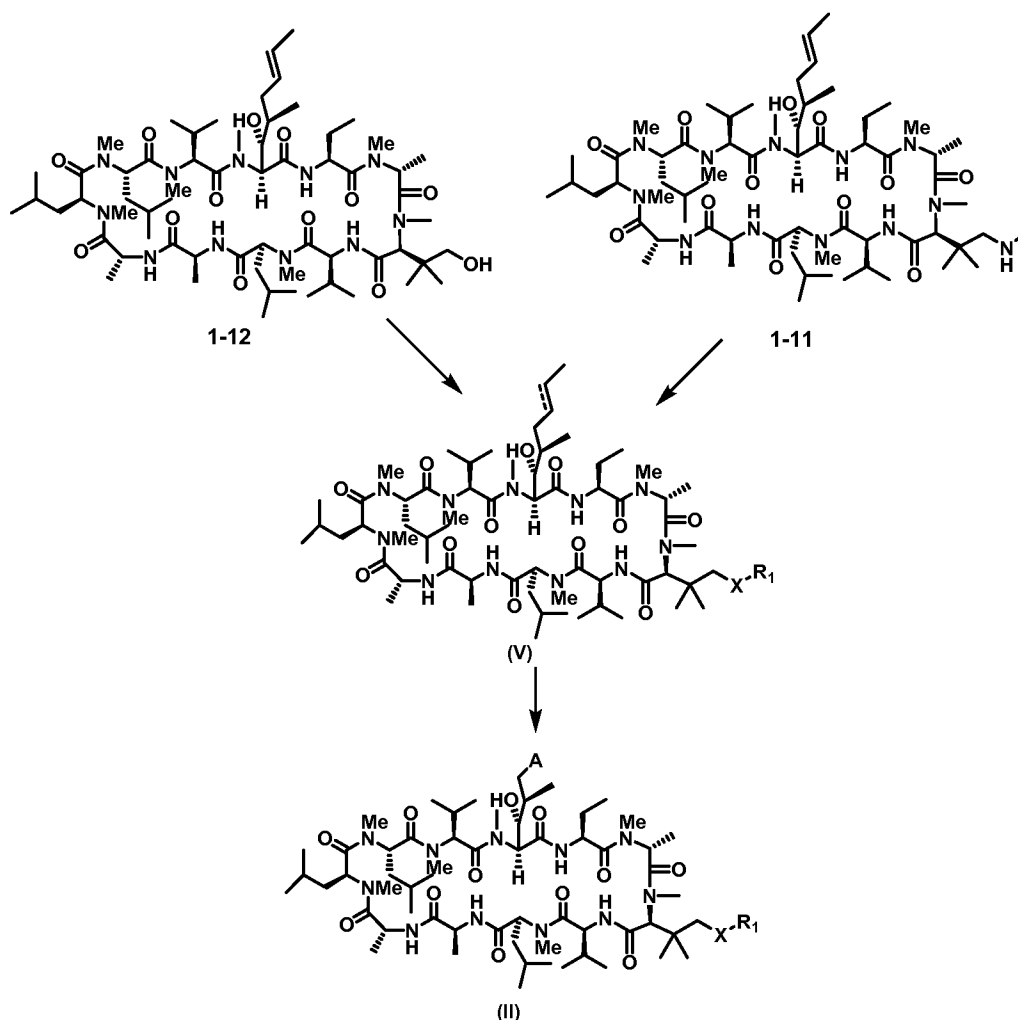
Scheme 2
