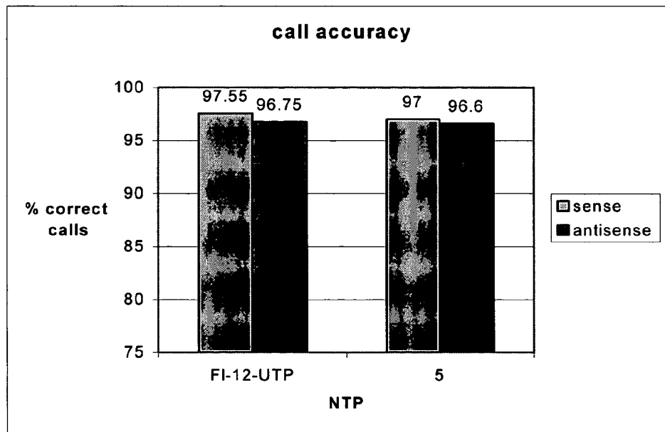
Chart 2. Call accuracy of NI-fluorescein-labeled 5-( \beta -D-ribofuranosyl)-2,4(1H,3H)-pyrimidinedione 5'-triphosphate 42a.
