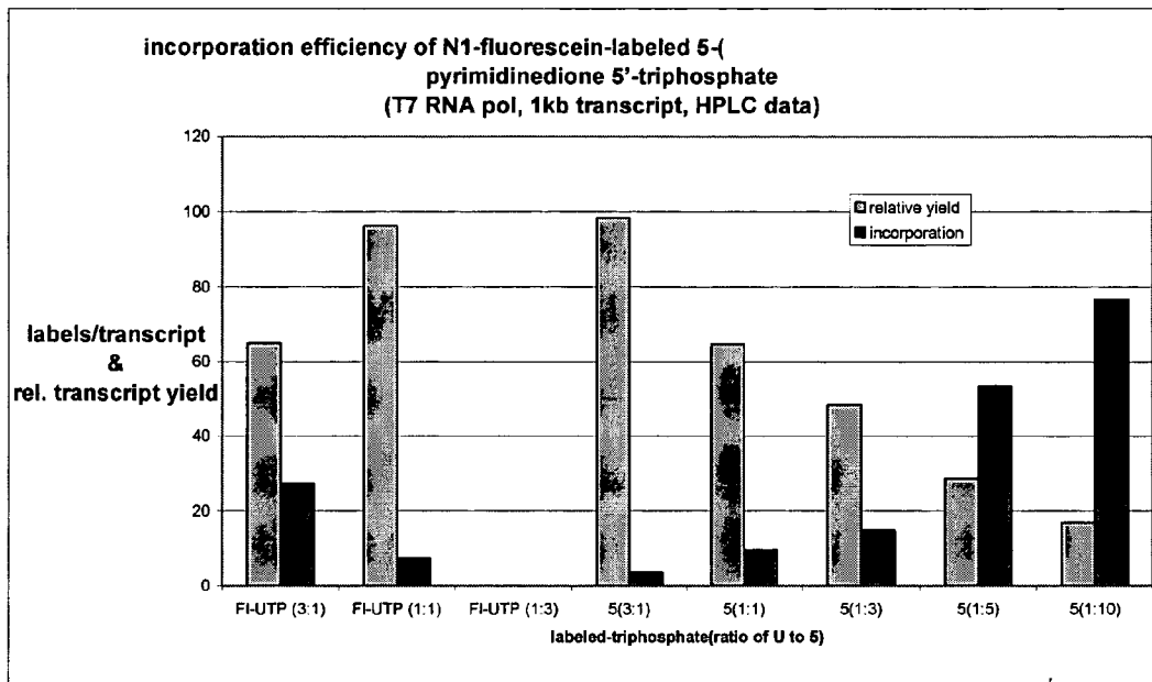
Chart 1. Incorporation efficiency of N1-fluorescein-labeled 5-( \beta -D-ribofuranosyl)-2,4(1H,3H)-pyrimidinedione 5'-triphosphate 42a , determined by HPLC
