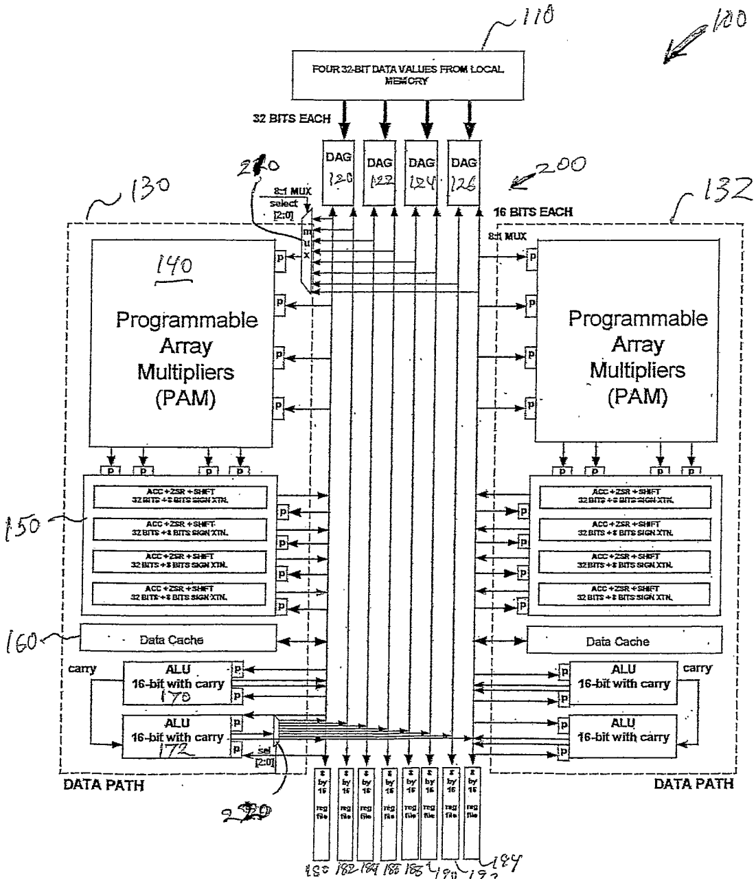
Figure 2. Data Path Detailed Block Diagram 1
