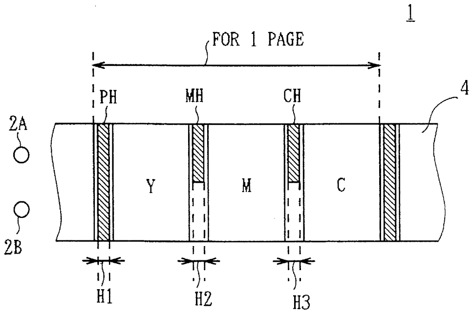
FIG. 1 (PRIOR ART)
