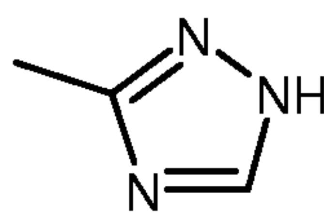
2H-tautomer
