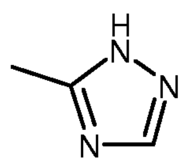
1H-tautomer
