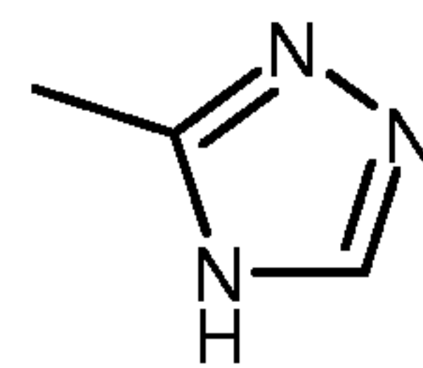
4H-tautomer.
