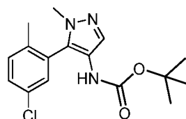
tert-Butyl 5-(5-chloro-2-methylphenyl)-1-methyl-1H-pyrazol-4-ylcarbamate
