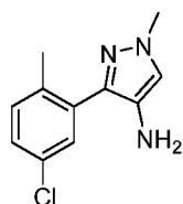
3-(5-Chloro-2-methylphenyl)-1-methyl-1H-pyrazol-4-amine
