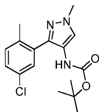
tert-Butyl 3-(5-chloro-2-methylphenyl)-1-methyl-1H-pyrazol-4-ylcarbamate
