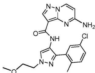
5-Amino-N-(3-(5-chloro-2-methylphenyl)-1-(2-methoxyethyl)-1H-pyrazol-4-yl)pyrazolo[1,5-a]pyrimidine-3-carboxamide
