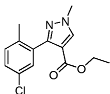
Ethyl 3-(5-chloro-2-methylphenyl)-1-methyl-1H-pyrazole-4-carboxylate
