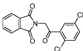
2-(2-(2,5-Dichlorophenyl)-2-oxoethyl)isoindoline-1,3-dione
