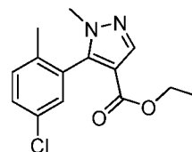
Ethyl 5-(5-chloro-2-methylphenyl)-1-methyl-1H-pyrazole-4-carboxylate
