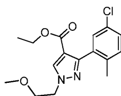
Ethyl 3-(5-chloro-2-methylphenyl)-1-(2-methoxyethyl)-1H-pyrazole-4-carboxylate
