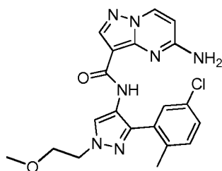
5-Amino-N-(3-(5-chloro-2-methylphenyl)-1-(2-methoxyethyl)-1H-pyrazol-4-yl)pyrazolo[1,5-a]pyrimidine-3-carboxamide
