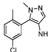
5-(5-Chloro-2-methylphenyl)-1-methyl-1H-pyrazol-4-amine
