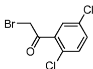
2-Bromo-1-(2,5-dichlorophenyl)ethanone
