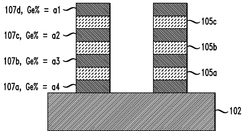
FIG. 1B CROSS FIN VIEW
