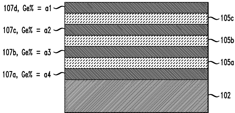
FIG. 1A CROSS GATE VIEW
