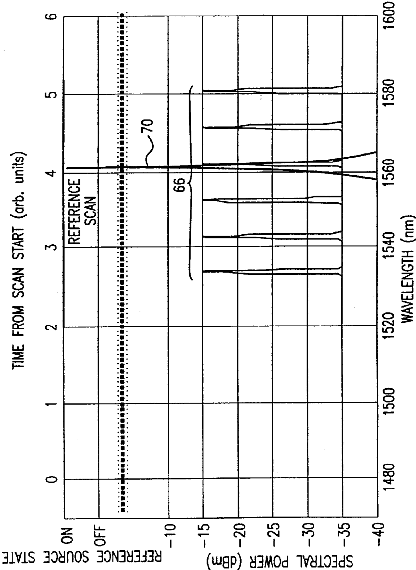
WDM SIGNAL AND MONITOR SPECTRA AND REFERENCE SIGNAL TEMPORAL MODULATION
