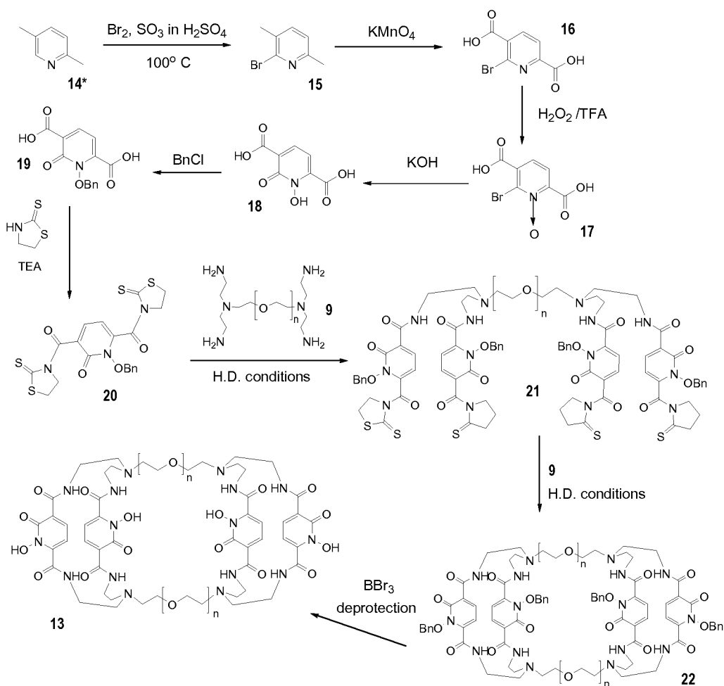
Scheme 2
