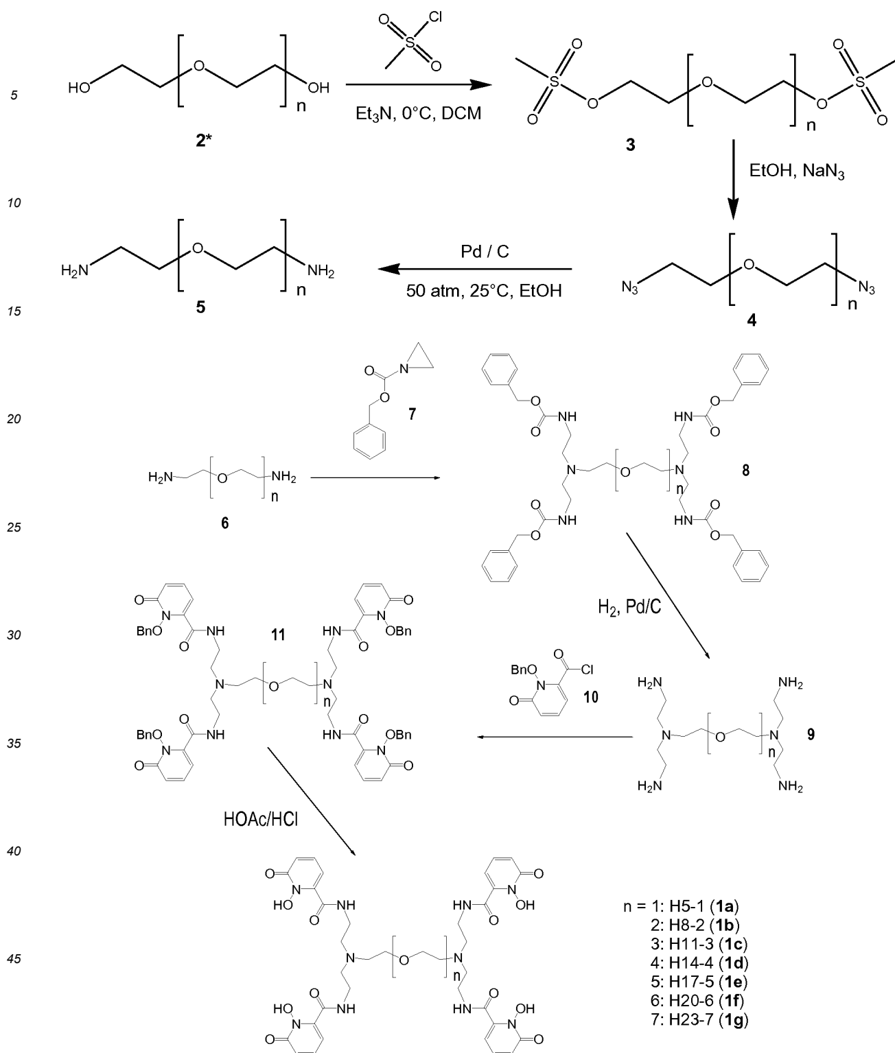
Scheme 1
