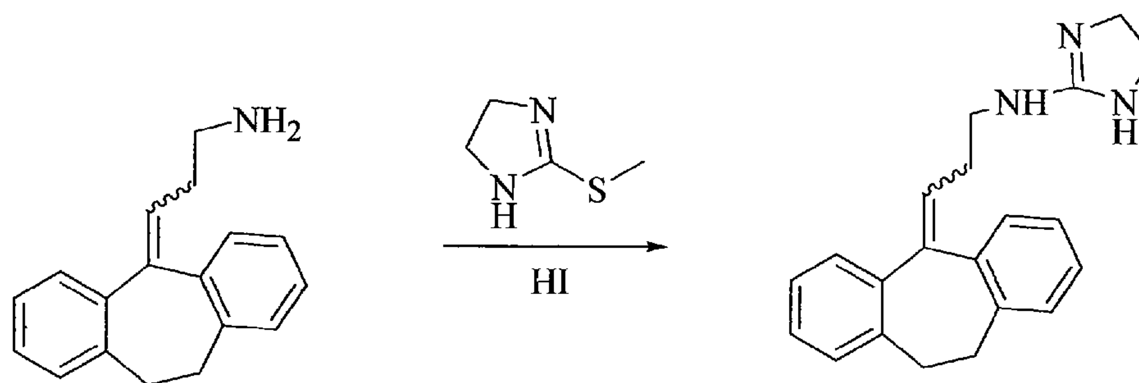
Scheme 5
