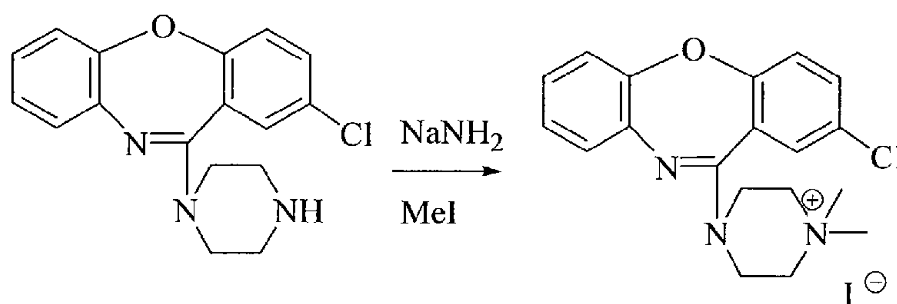
Scheme 1
