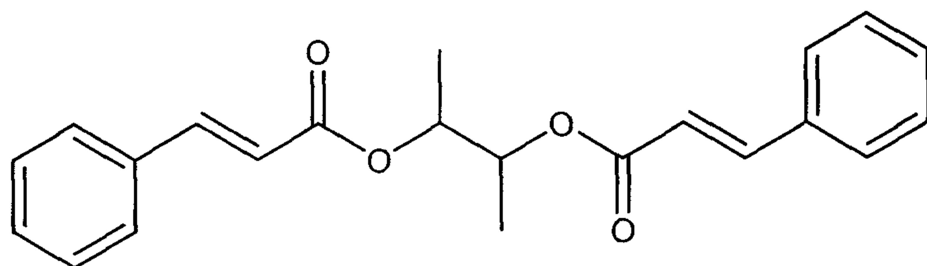
trans -cinnamic acid-2,3-butanediol diester, of the formula
