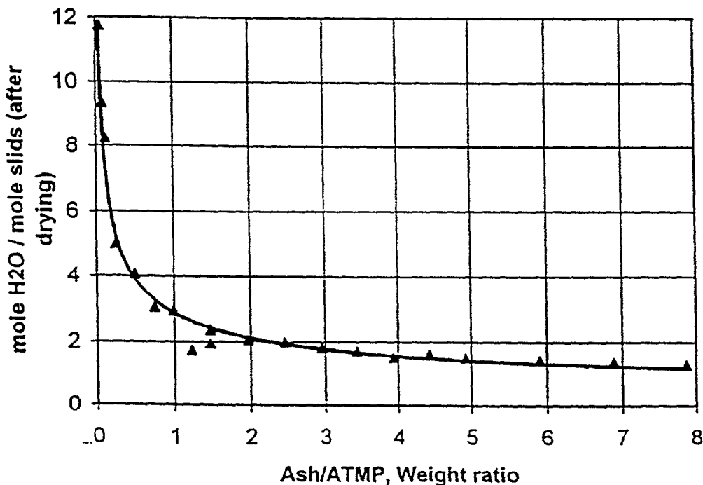
FIGURE 4 Drying of Ash-ATMP Solutions
