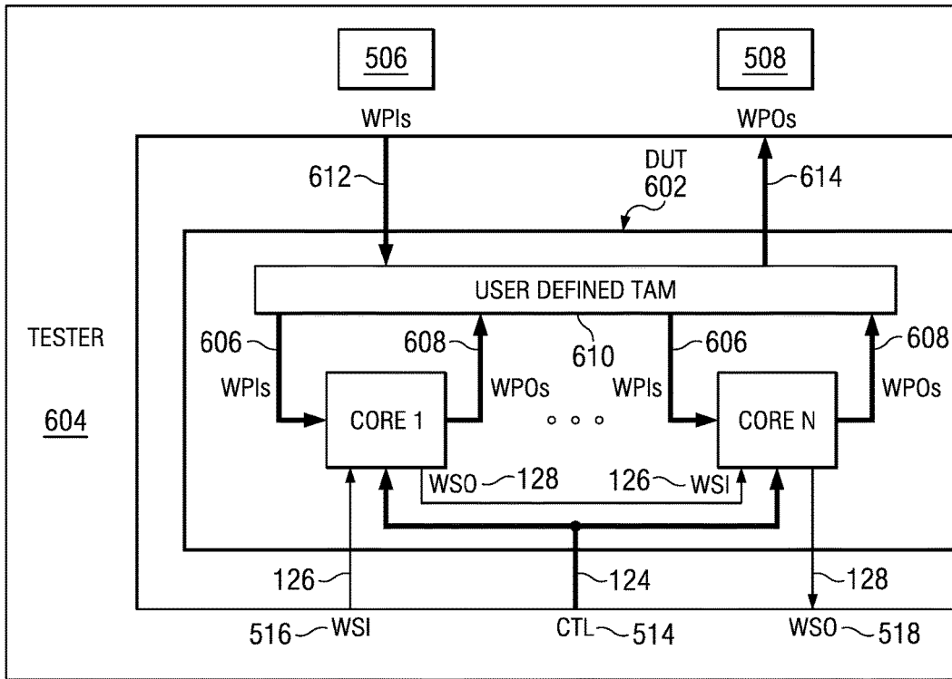
FIG. 6 (PRIOR ART)
