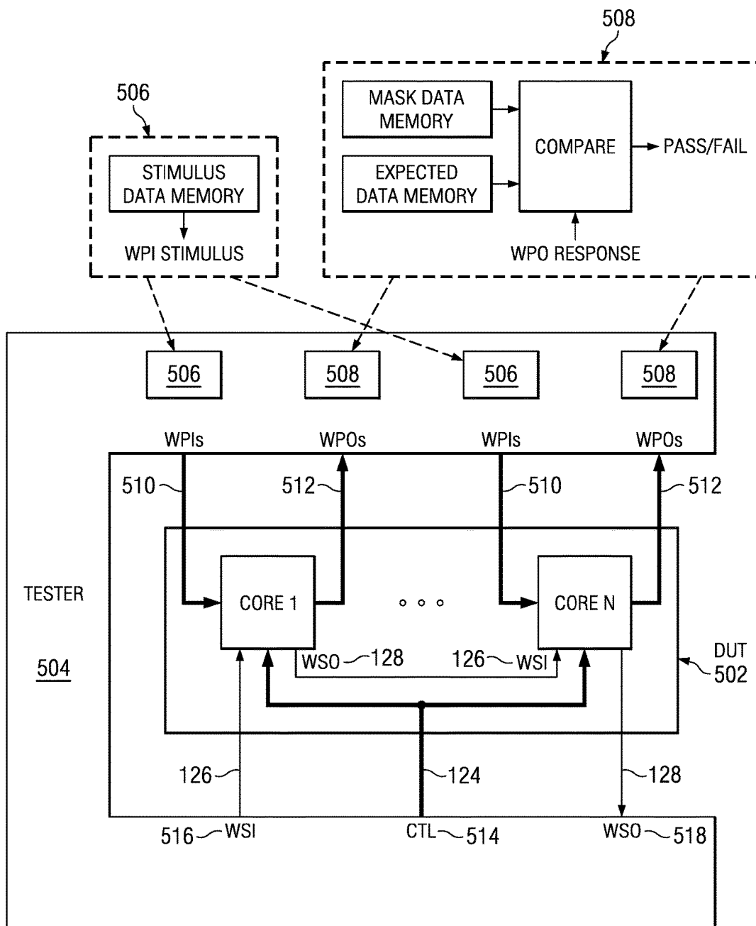
FIG. 5 (PRIOR ART)
