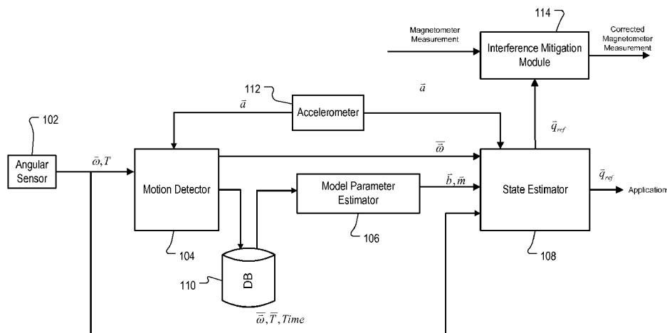
Sensor Measurement Calibration System 100
