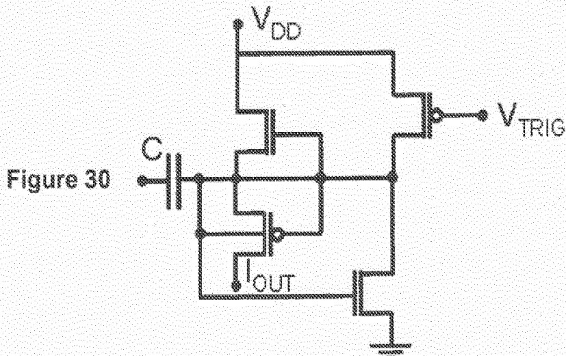
Compact CMOS Programmable Trigger Circuit
