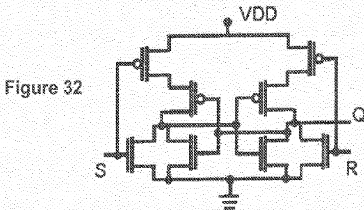
Compact CMOS Trigger Circuit
