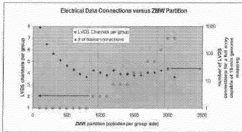
LVDS connections to support very high data rates
