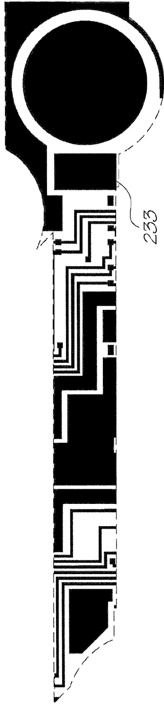
Metal 2 mask
