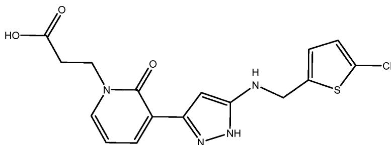
(Compound 2).
