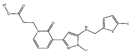
(Structure II)
