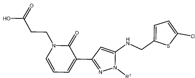
(Structure I)
