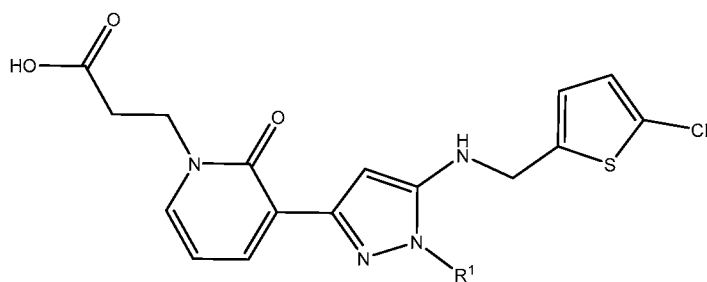
(Structure I)
