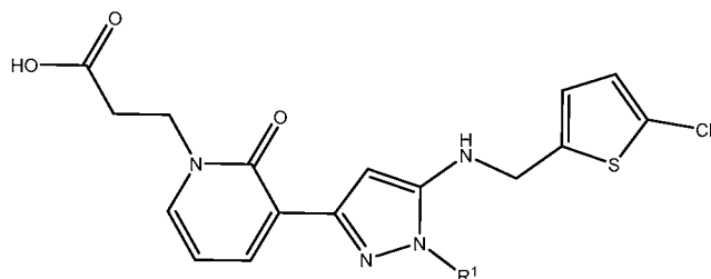
(Structure I)
