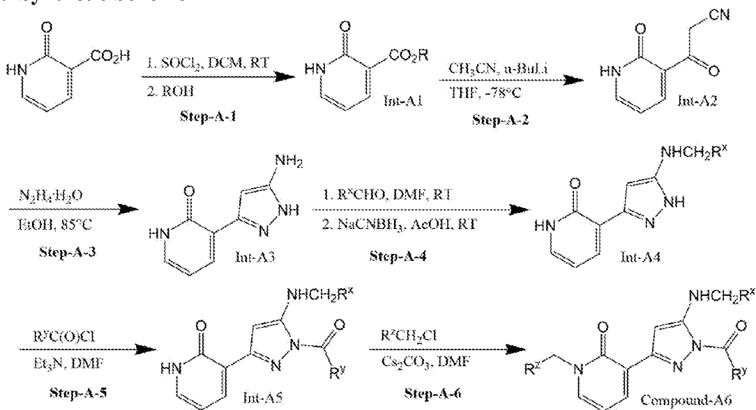
Step-A-1 – Synthesis of Exemplary Int-A1
