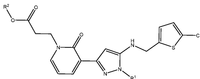
(Structure II)
