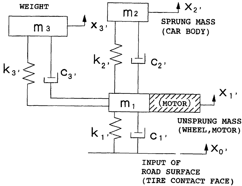
FIG. 73 (b) PRIOR ART
