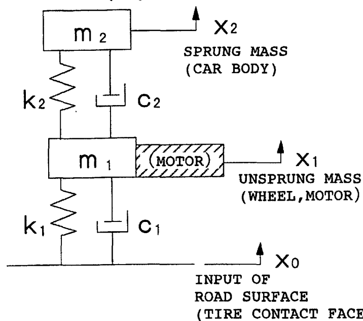
FIG. 72 (b) PRIOR ART
