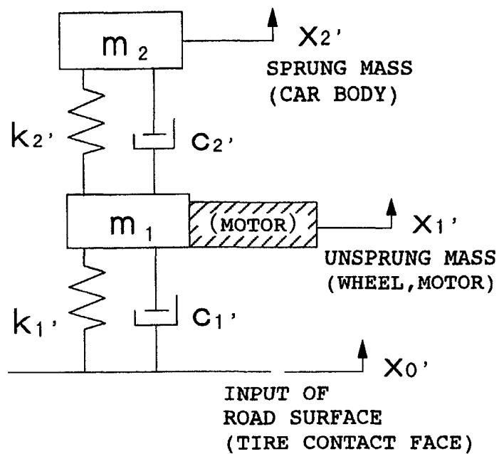
FIG. 72 (b) PRIOR ART
