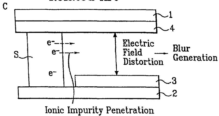
FIG.3 Related Art
