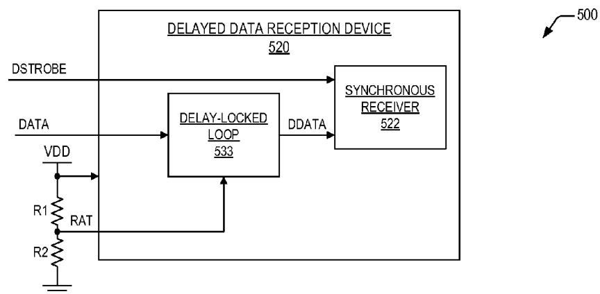
APPARATUS FOR DELAYED SYNCHRONOUS DATA RECEPTION
