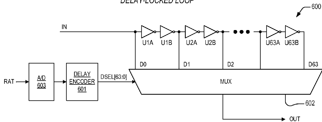
DELAY-LOCKED LOOP
