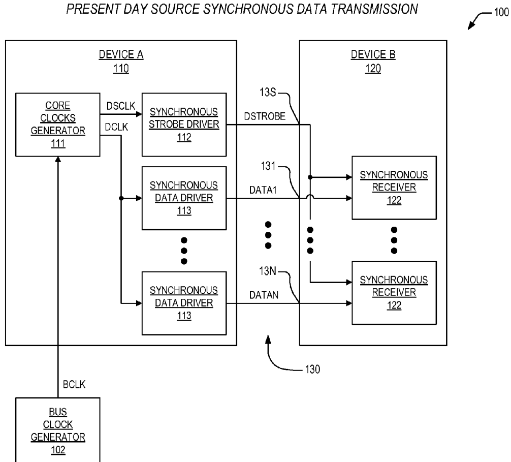
FIG. 1 (Prior Art)
