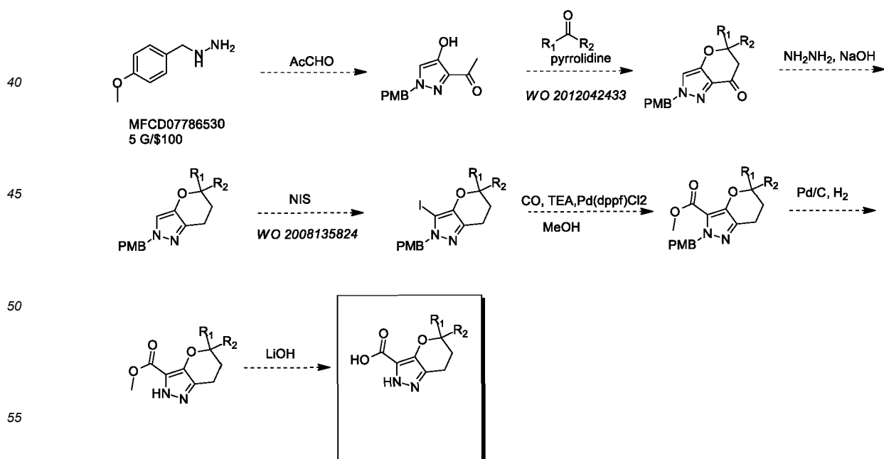
Scheme 7
