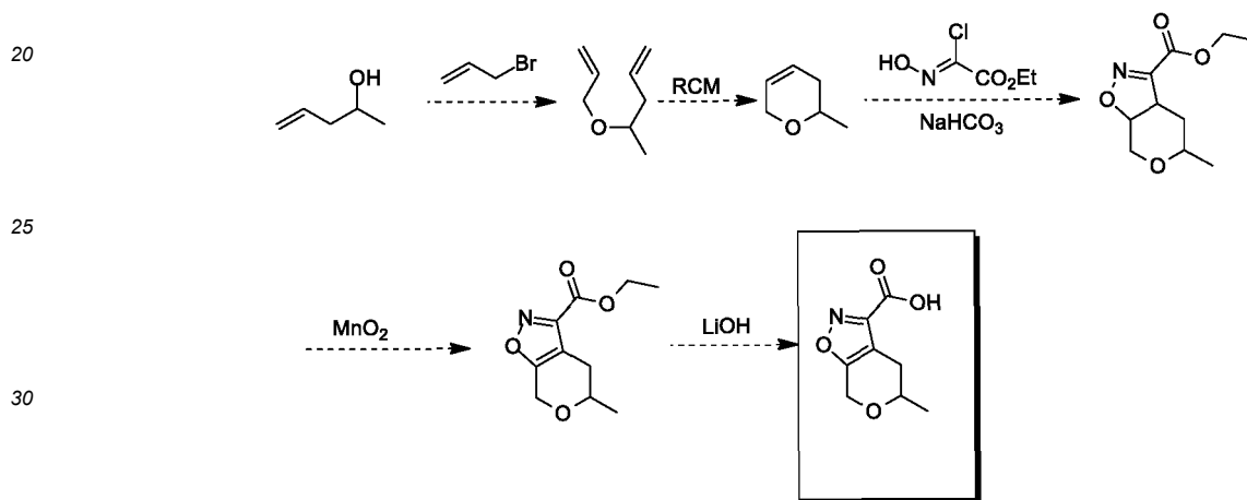
Scheme 6
