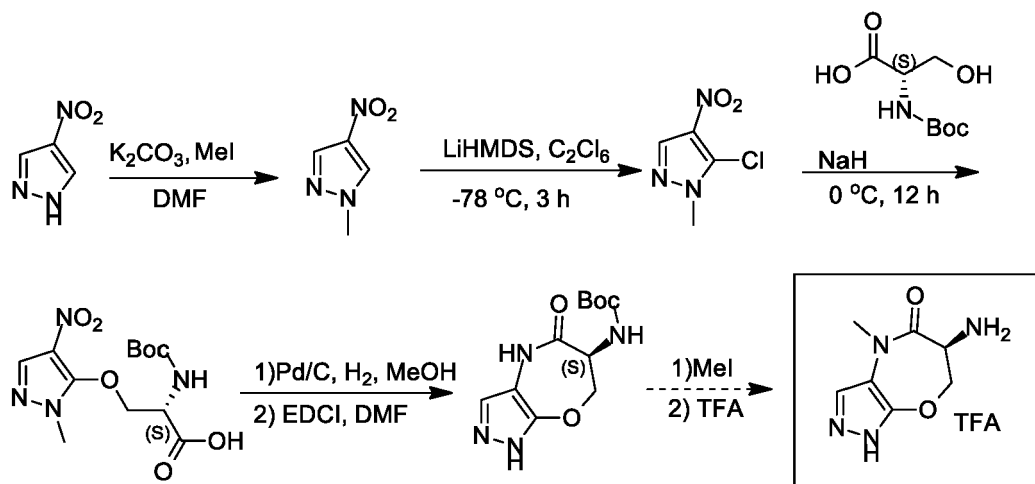
Scheme 14
