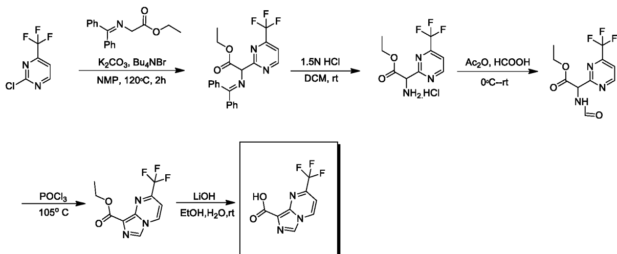
Scheme 12
