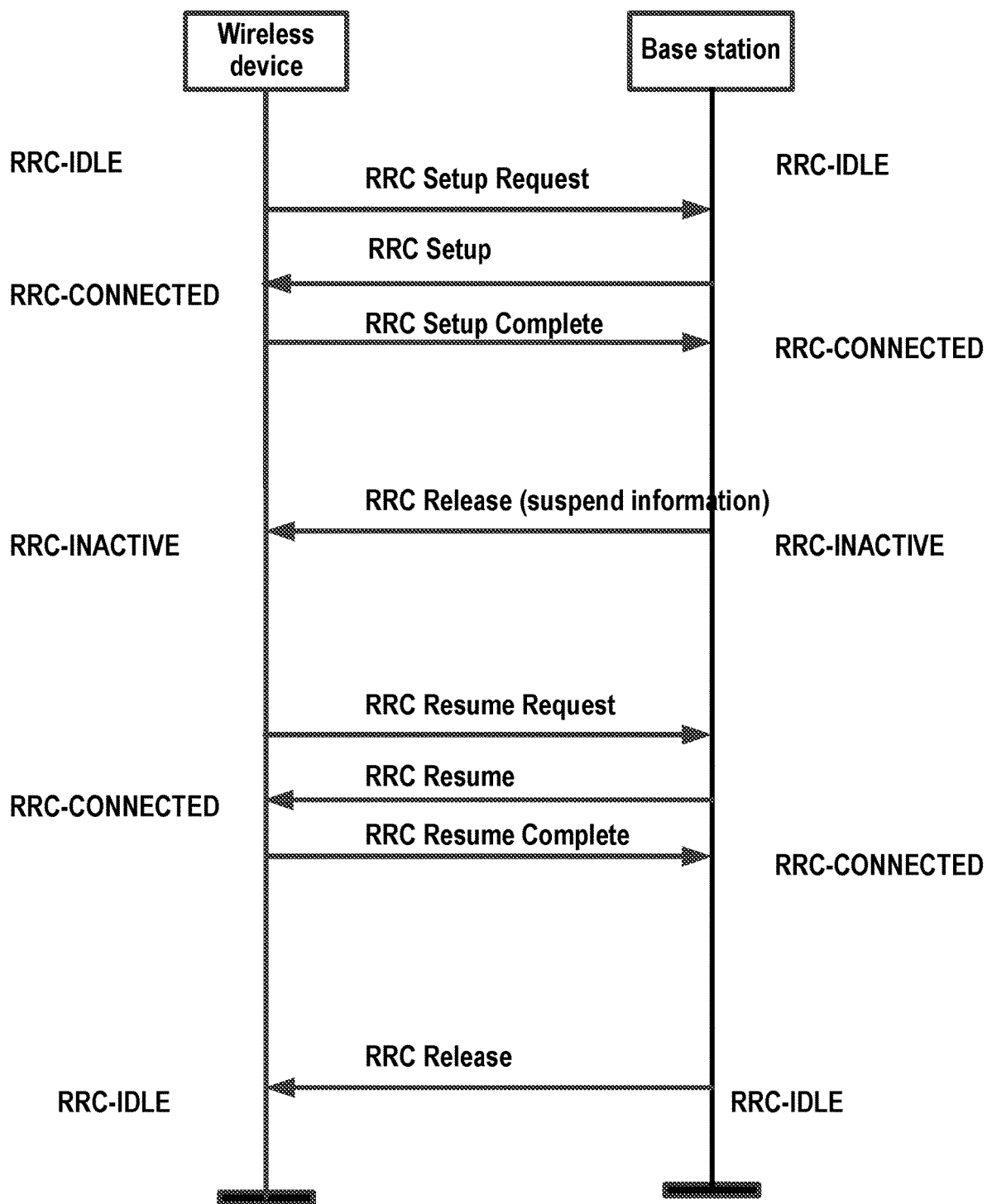
Call flow for RRC state transition
